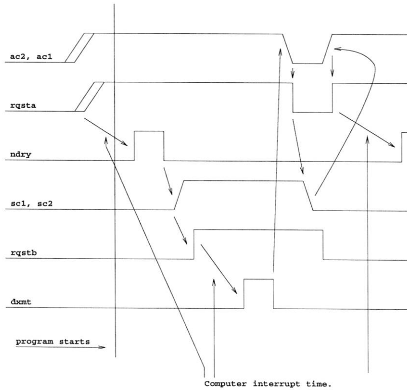
Figure A3: Interface Timing
