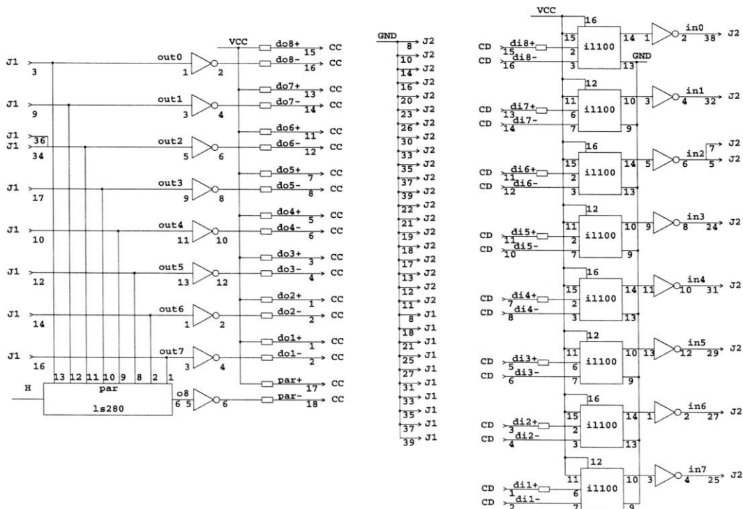
Figure A1: Interface between Linotron 202 and DR11-C
