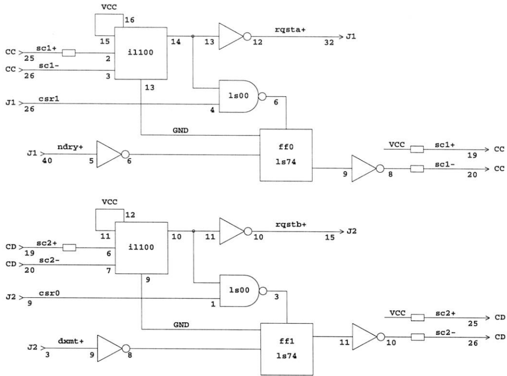
Figure A2: Interface Signals
